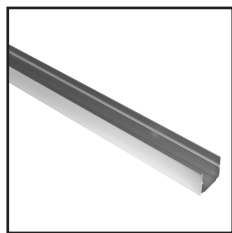
Aluminium Profile Order Code : 8982010-01 Dimension : L1000xW20.5xH17.6mm Material : aluminium Color : silver
