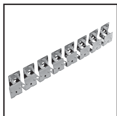
Curved Profile Order Code : 8982010-02 Dimension : L500xW17xH15mm Material : stainless steel Color : silver
