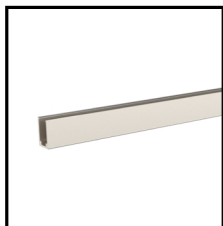
Aluminium Profile Order Code: 8931818-01 Dimension: L1000xW19.8H16.9 Material: aluminium Color: silver
