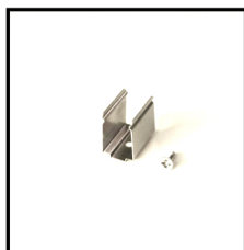
Mounting Clips Order Code: 8981616-03 Dimension: L20xW16.6xH12.4mm Material: stainless steel Color: silver Each meter led strips needs 2 clips + 2 screws
