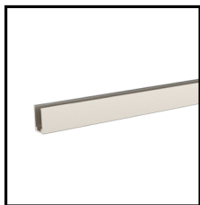
Aluminium Profile Order Code: 8981515-01 Dimension: L1000xW20.5xH17.6mm Material: aluminium Color: silver
