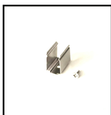
Mounting Clips Order Code: 8981515-05 Dimension: L20xW16.6xH12.4mm Material: stainless steel Color: silver Each meter led strips needs 2 clips + 2 screws
