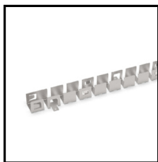
Curved Profile Order Code: 8981515-02 Dimension: L500xW17xH15mm Material: stainless steel Color: silver
