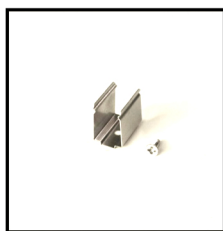
Mounting Clips Order Code: 8981212-03 Dimension: L11.6xW8xH7.6mm Material: stainless steel Color: silver Each meter led strips needs 2 clips + 2 screws
