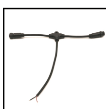
IP67 T Type Connector Order Code: 8981515-11 Wire Gauge: 0.326mm 2 /22AWG Protection: IP67 (Mated)
