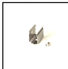
Mounting Clips Order Code: 8981515-05 Dimension:L20xW16.6xH12.4mm Material: stainless steel Color: silver Each meter led strips needs 2 clips + 2 screws
