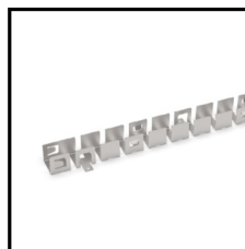
Curved Profile Order Code: 8981515-02 Dimension:L500xW17xH15mm Material: stainless steel Color: silver
