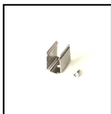
Mounting Clips Order Code: 8941212-03 Dimension: L11.6xW14xH14.6mm Material: stainless steel Color: silver Each meter led strips needs 2 clips + 2 screws
